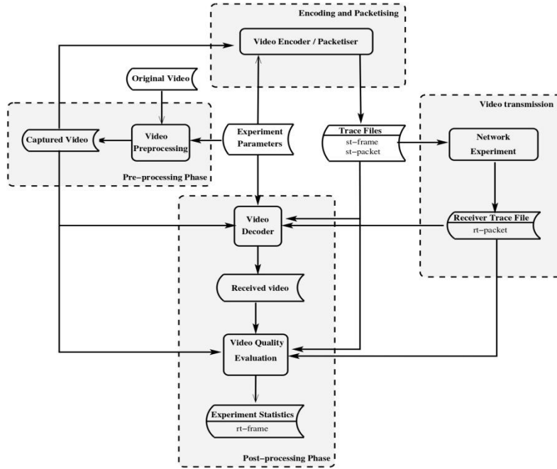
Fig. 5. SenseVid Architecture (redrawn from Maimour, 2018b)
