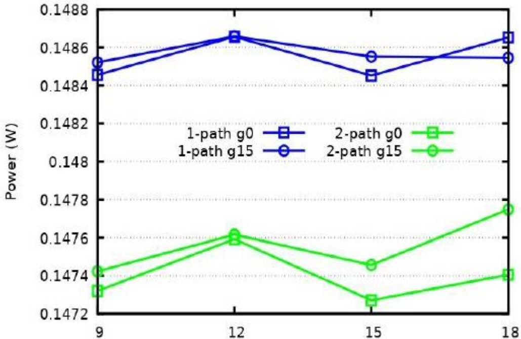
Fig 9. S Mean Power Consumption.
