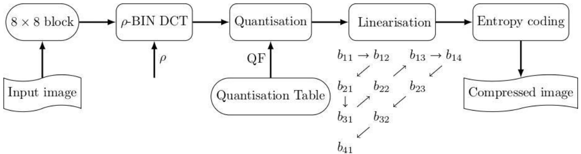
Fig. 2. M-frame block encoding sequence ( \rho = 4 ).
