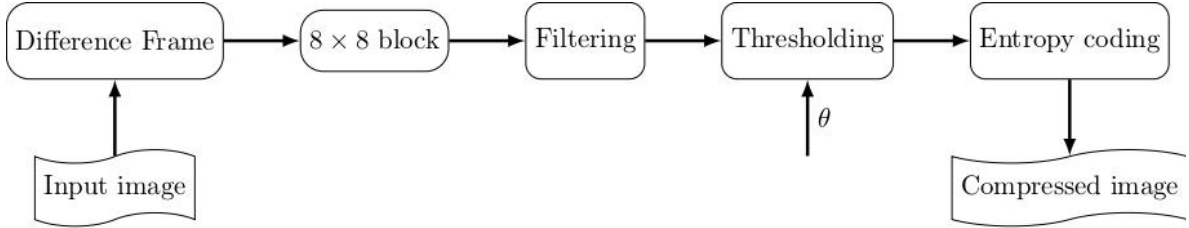
Fig 3. S-frame encoding sequence.
