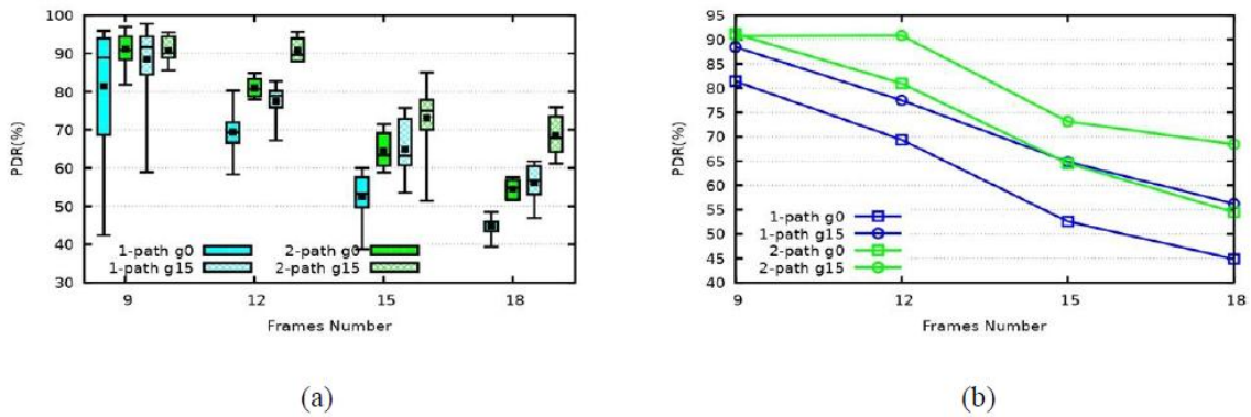
Fig. 6. PDR (a) distribution (b) mean values
