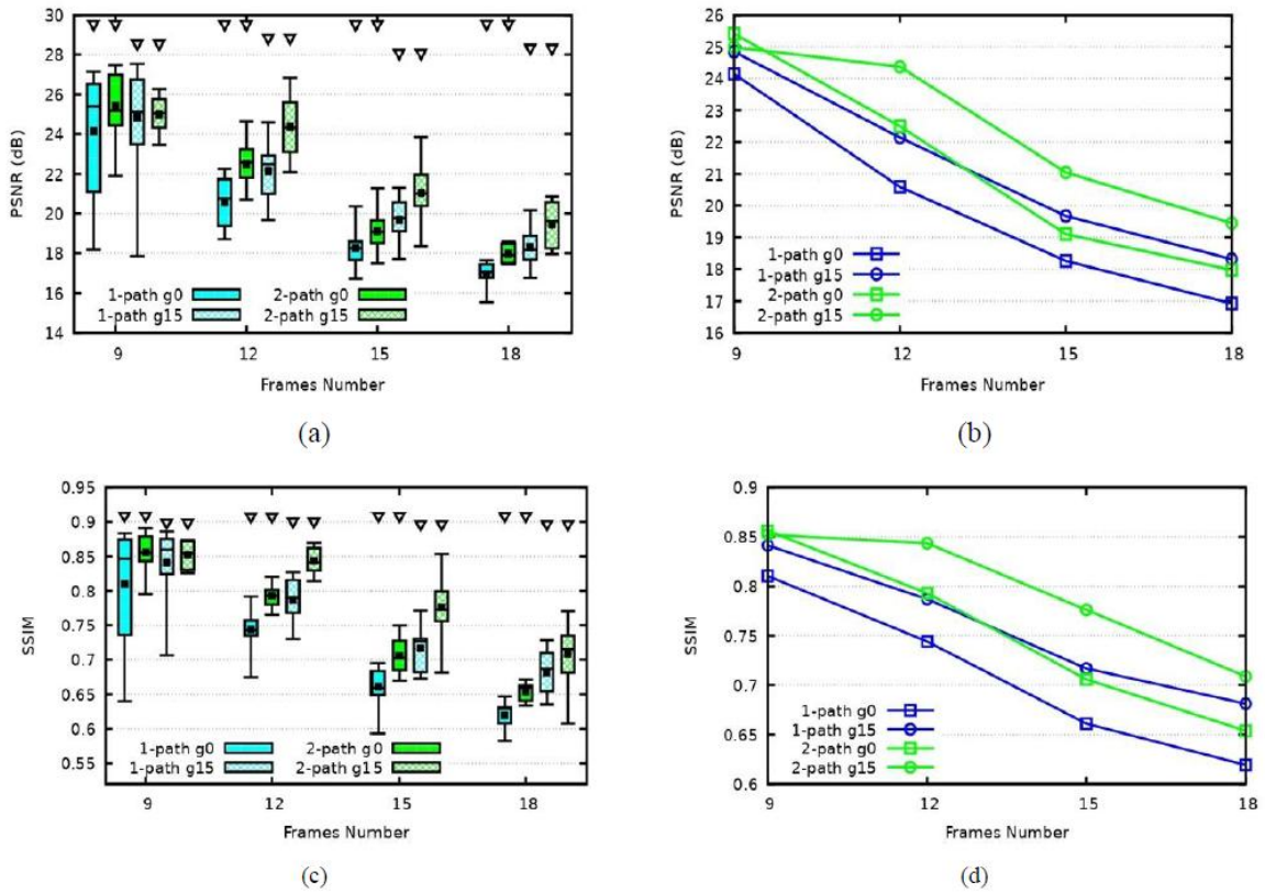
Fig 7. Obtained Images Quality (a) PSNR distribution, (b) PSNR mean, (c) SSIM distribution, (d) SSIM mean.
